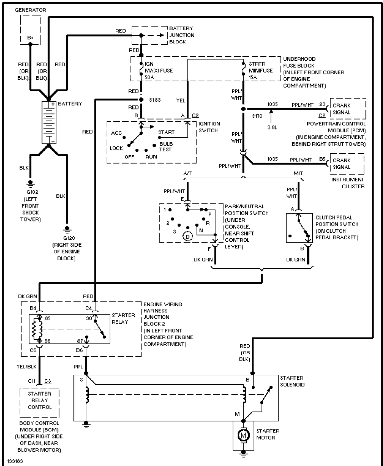
Starting Circuit
