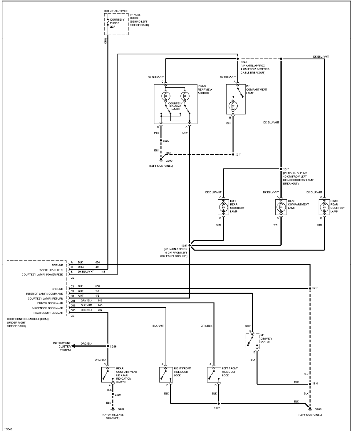
Courtesy Lamps Circuit, Convertible
